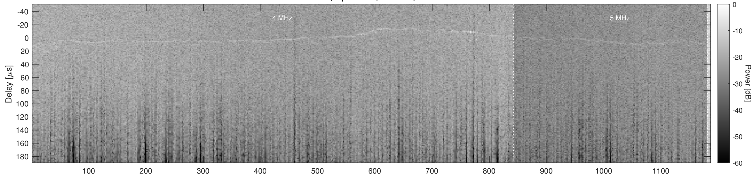
Orbit 10864, Optimized, Window, Channel 2
