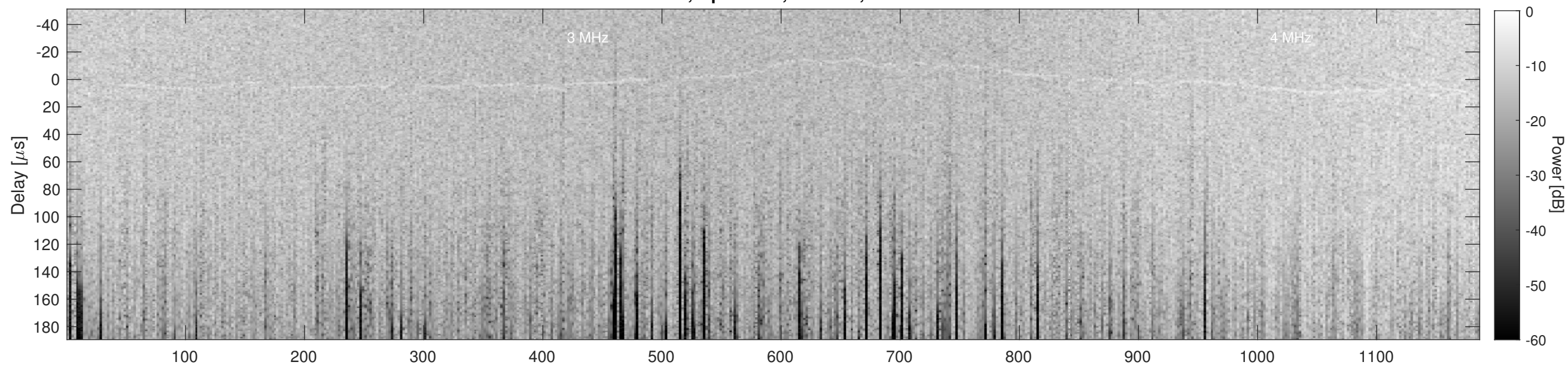
Orbit 10864, Cluttergram
