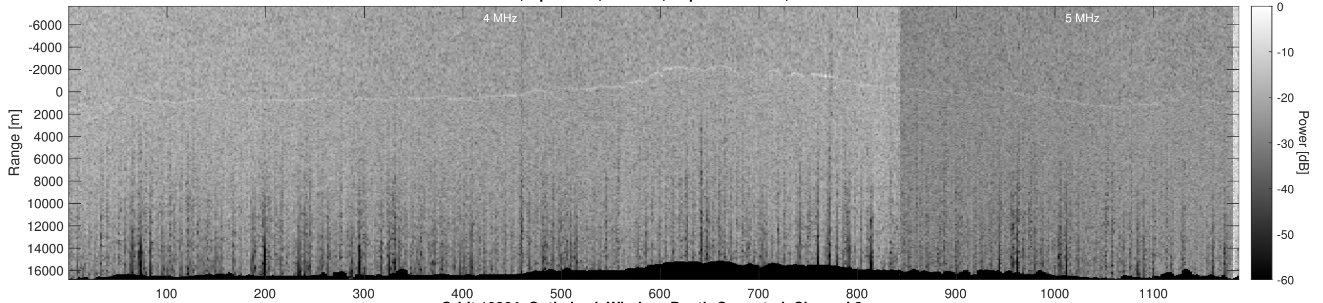
Orbit 10864, Optimized, Window, Depth-Corrected, Channel 2
