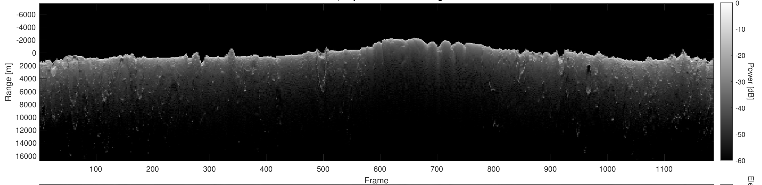
Orbit 10864, Depth-Corrected Cluttergram
