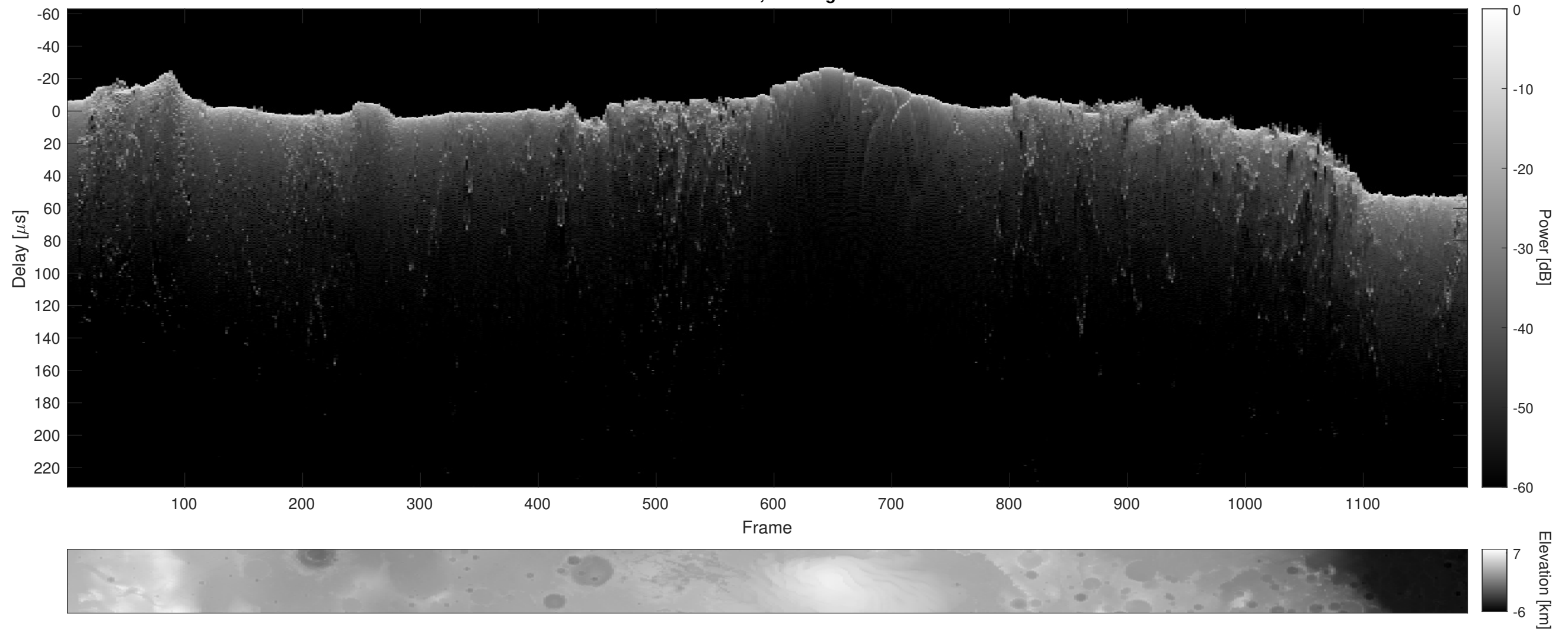
Orbit 10865, Cluttergram
