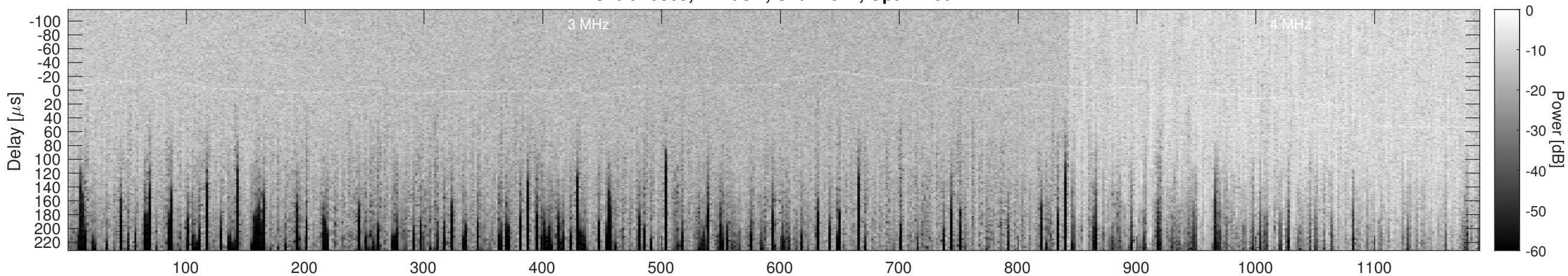
Orbit 10865, Cluttergram
