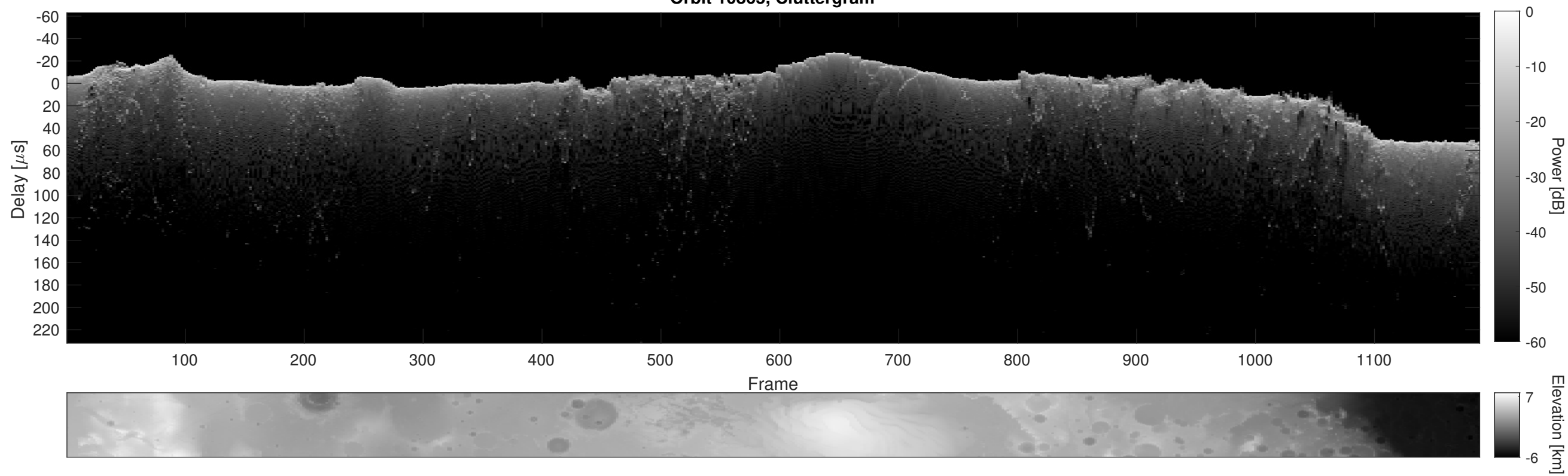
Orbit 10865, Cluttergram
