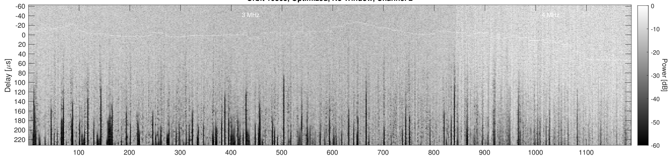
Orbit 10865, Cluttergram
