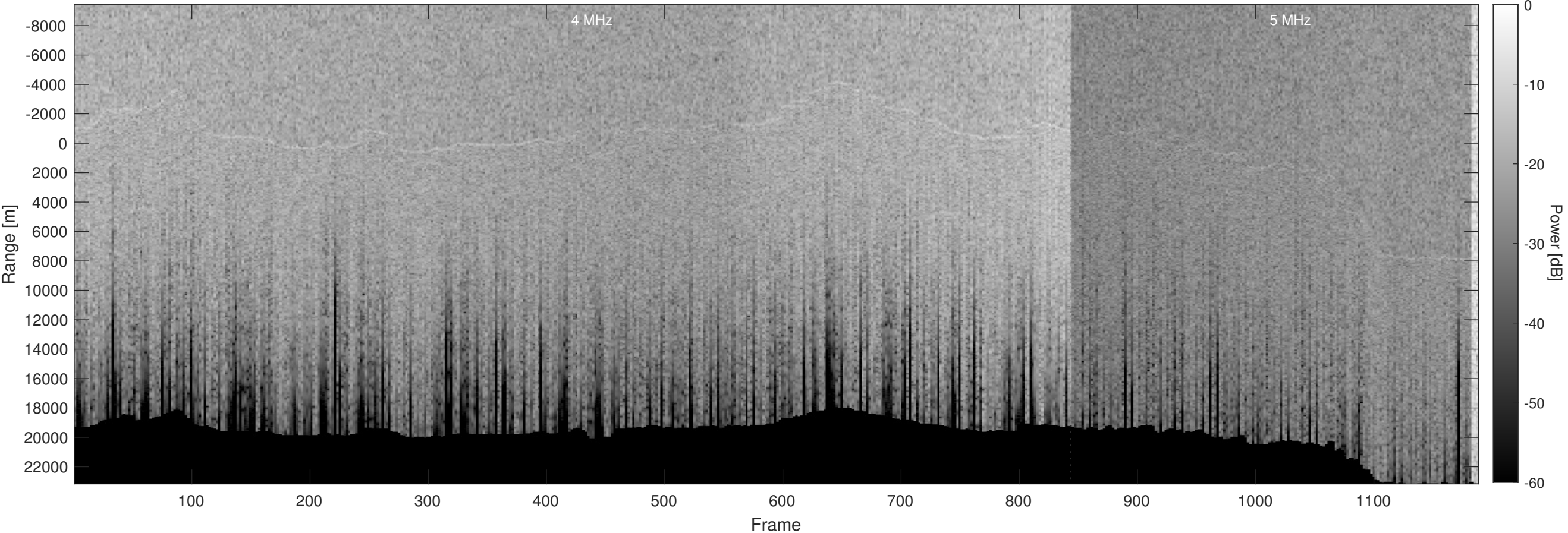
Orbit 10865, Optimized, Window, Depth-Corrected, Channel 2
