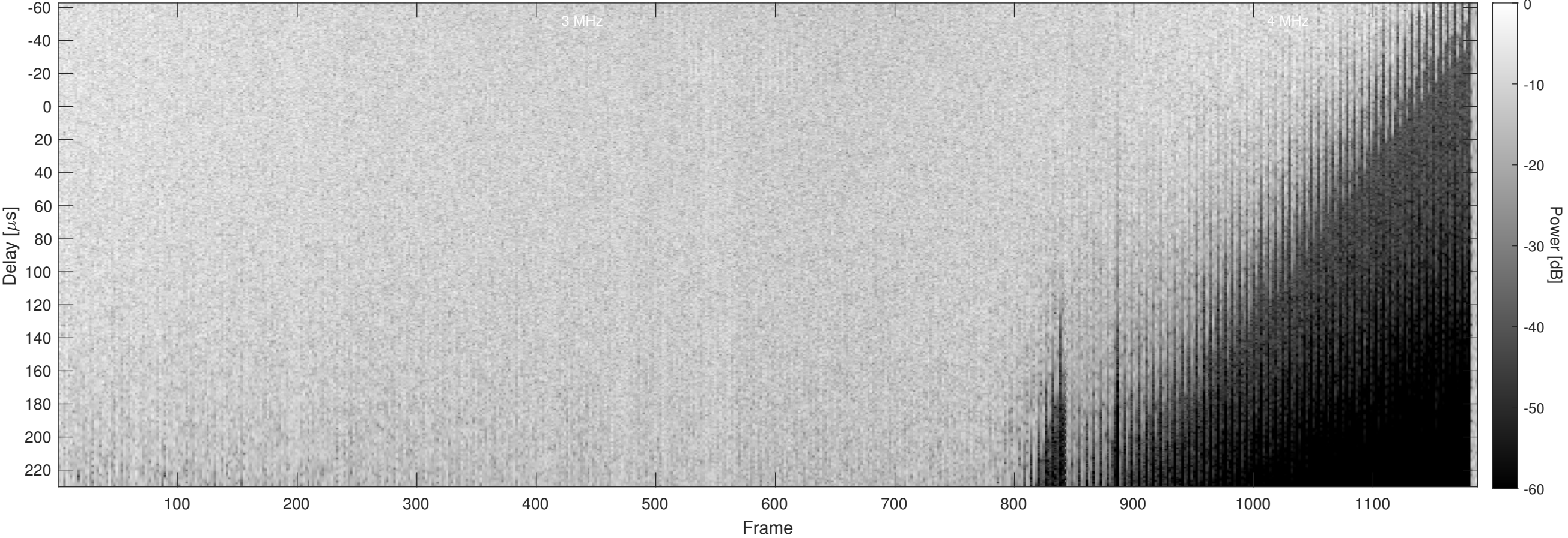
Orbit 10867, Chapman, No Window, Channel 2
