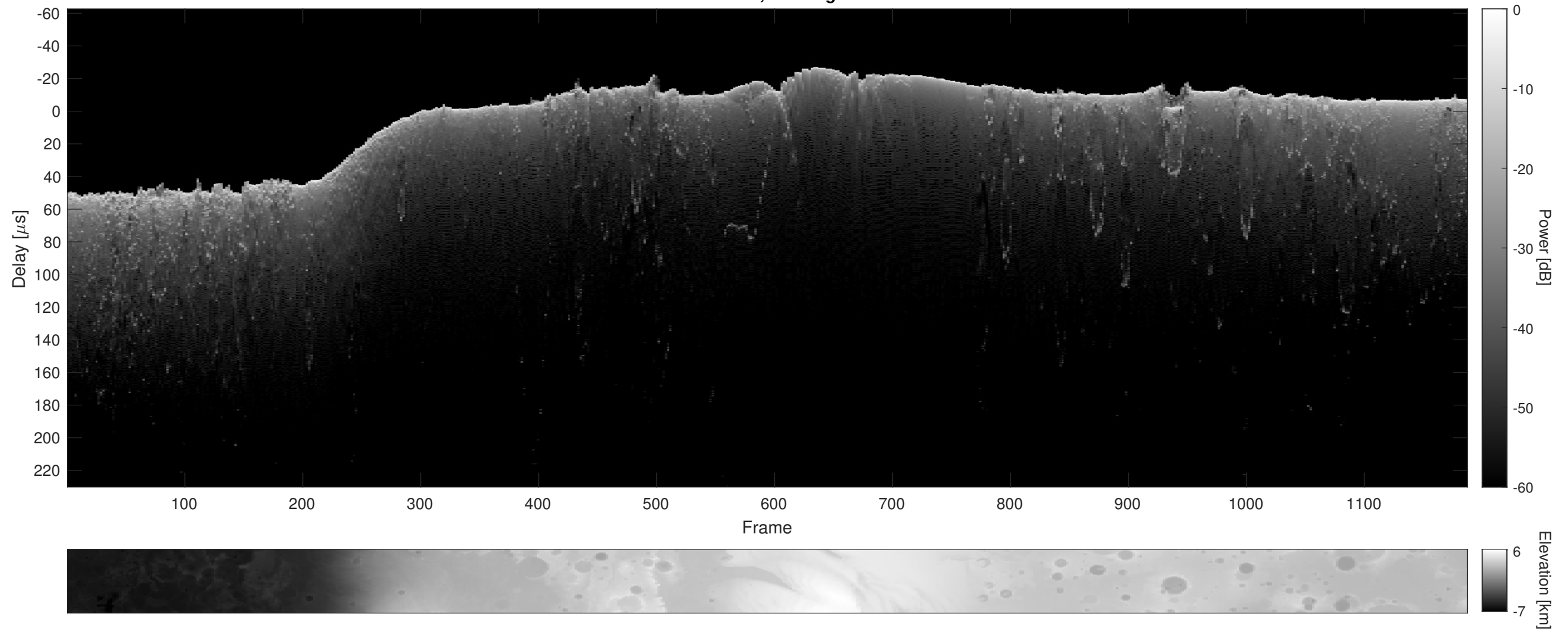
Orbit 10867, Cluttergram
