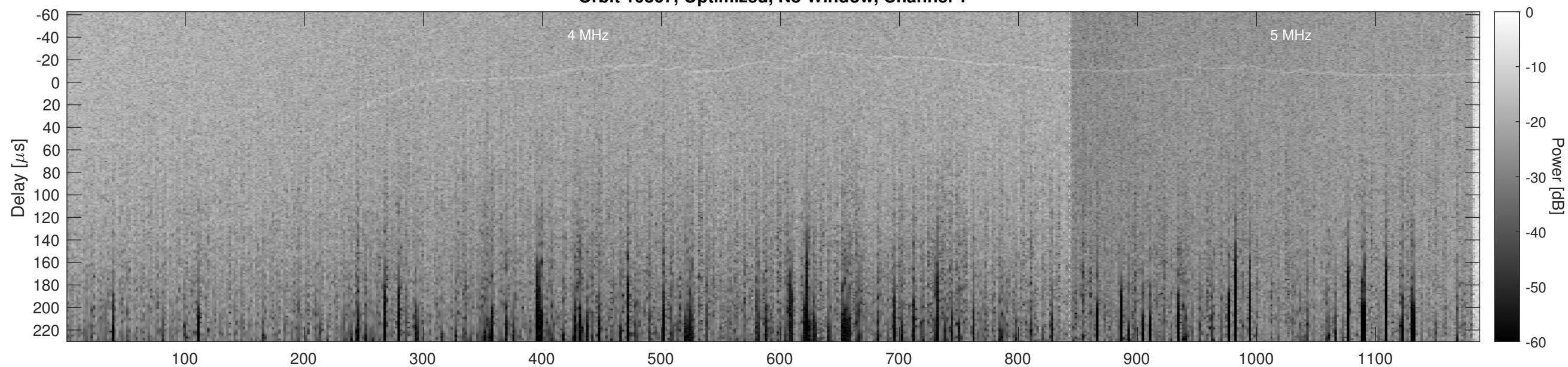
Orbit 10867, Optimized, No Window, Channel 2
