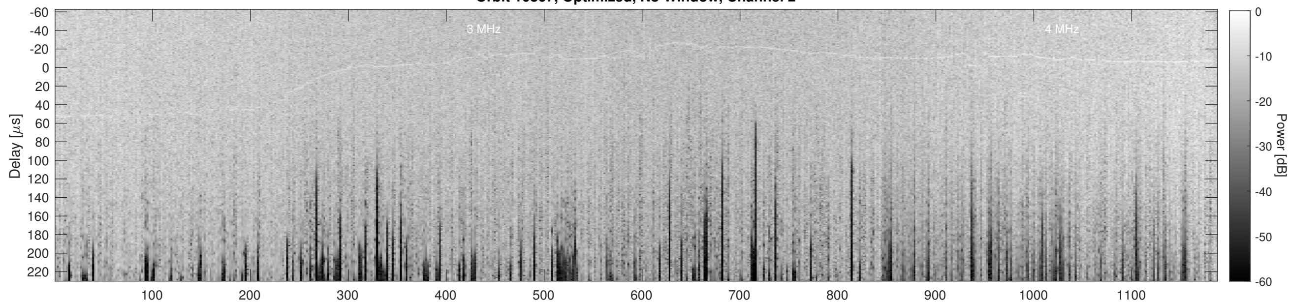
Orbit 10867, Cluttergram
