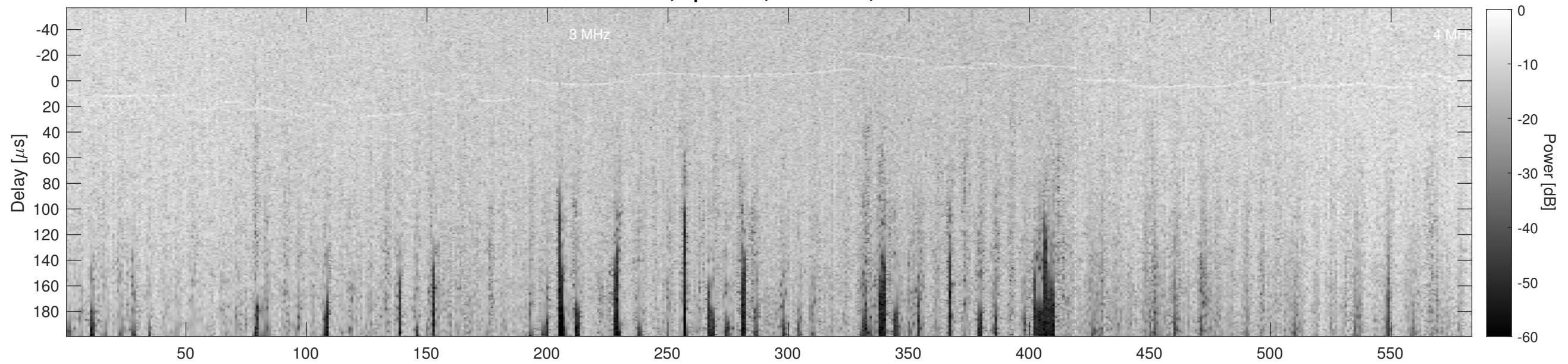
Orbit 10868, Cluttergram
