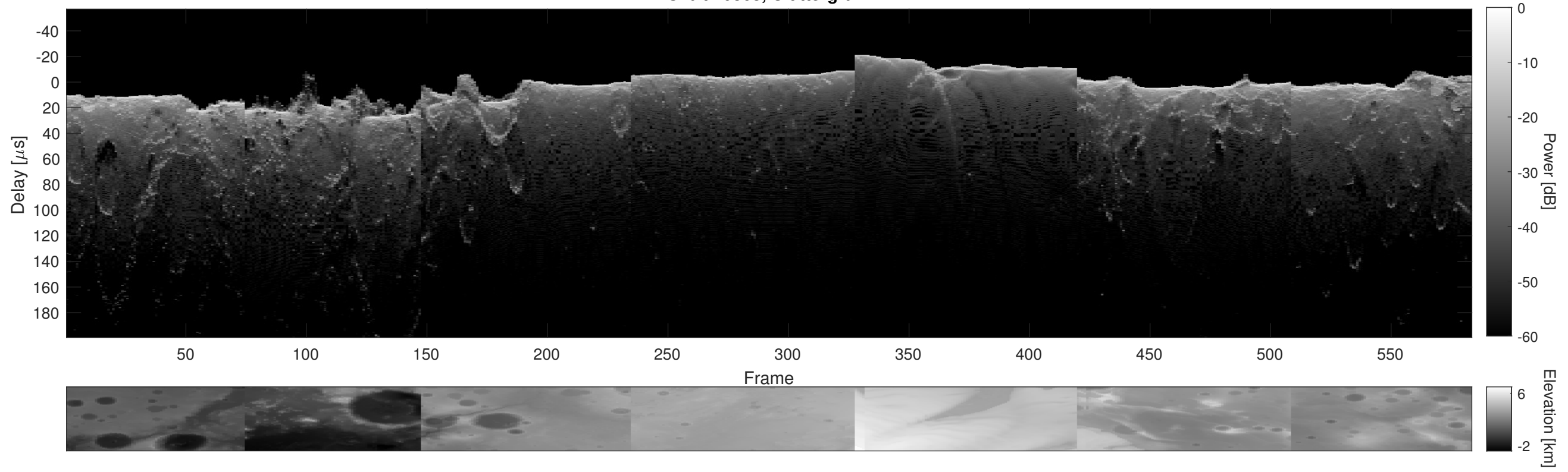
Orbit 10868, Cluttergram
