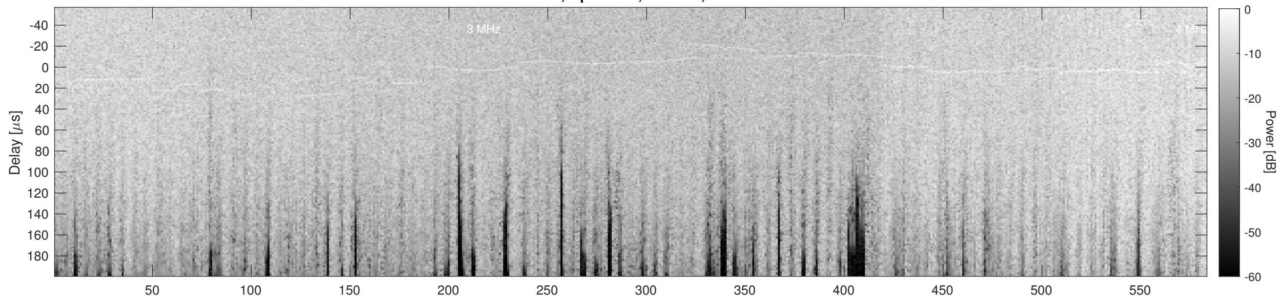
Orbit 10868, Cluttergram
