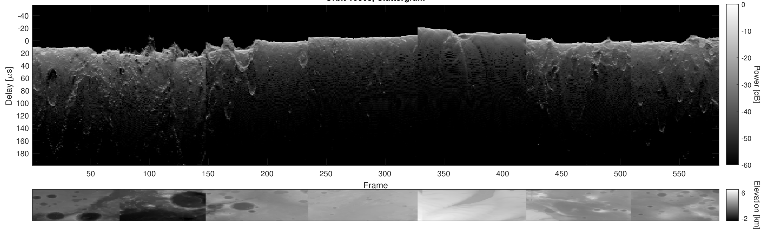
Orbit 10868, Cluttergram
