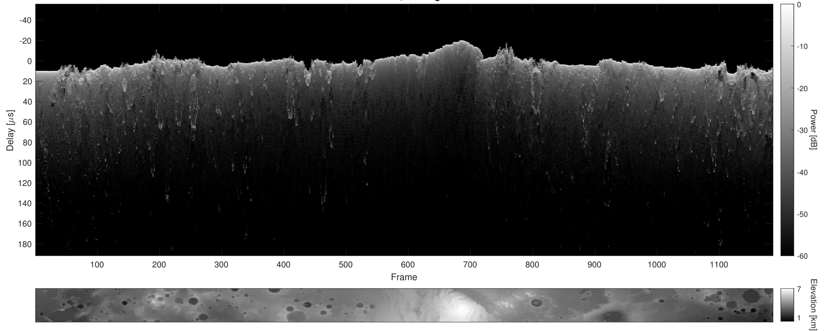
Orbit 10869, Cluttergram
