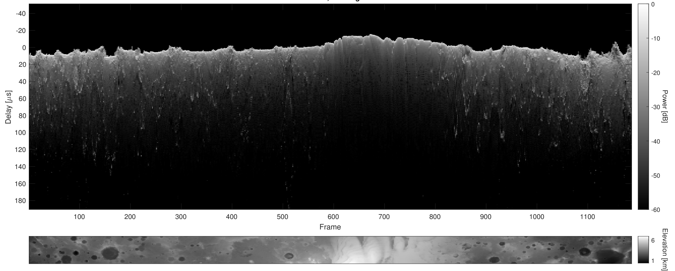
Orbit 10871, Cluttergram
