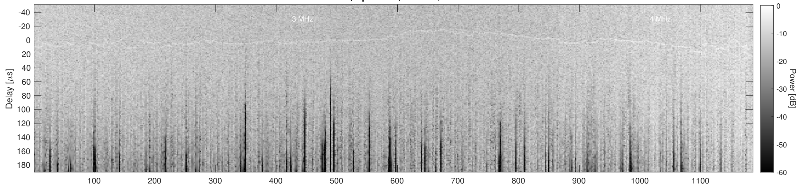
Orbit 10871, Cluttergram
