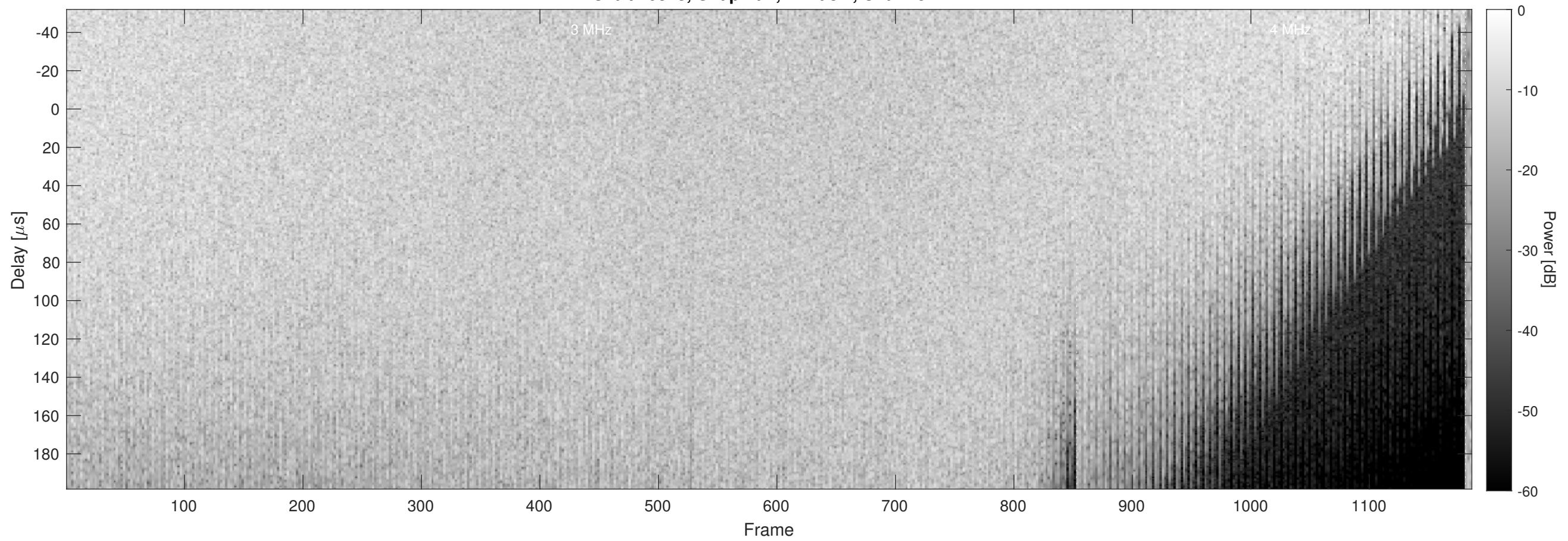
Orbit 10873, Chapman, Window, Channel 2
