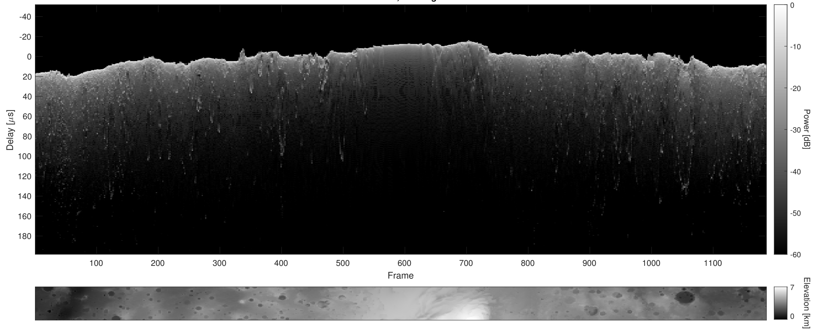
Orbit 10873, Cluttergram
