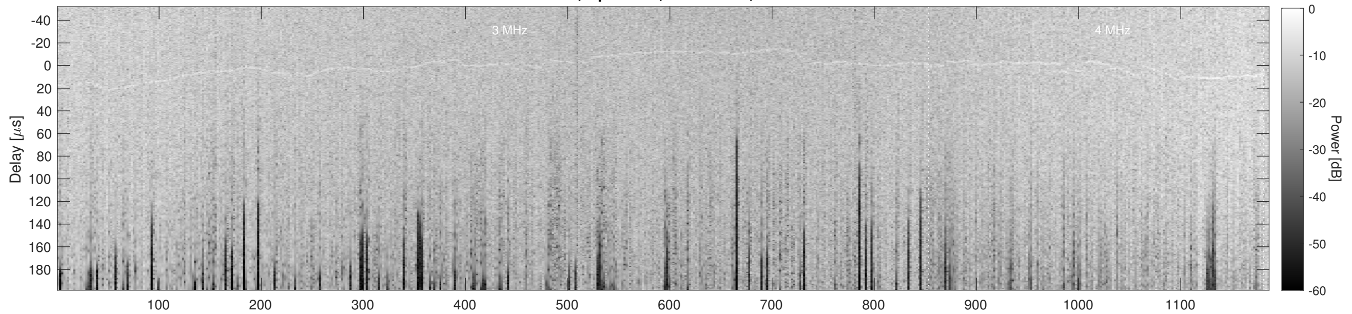
Orbit 10873, Cluttergram
