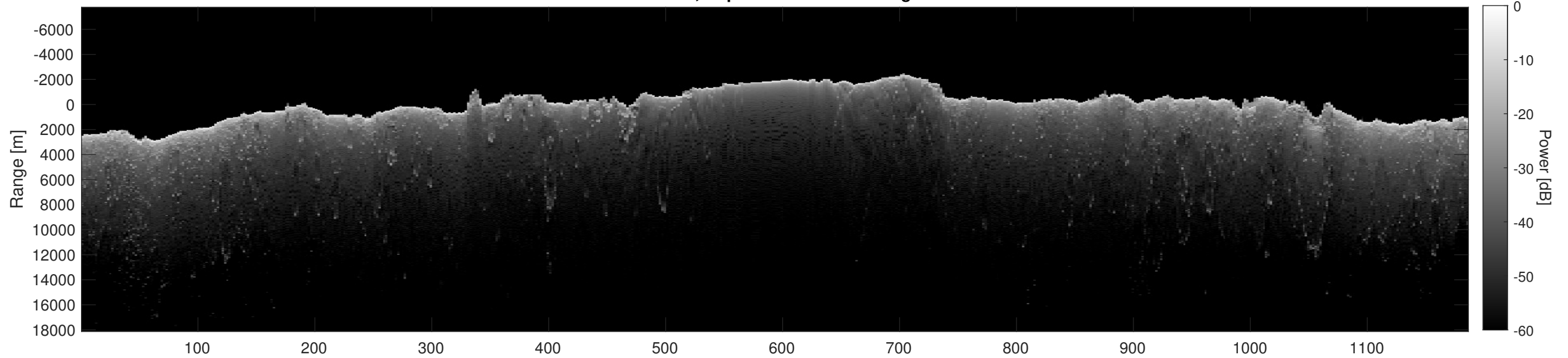
Orbit 10873, Depth-Corrected Cluttergram
