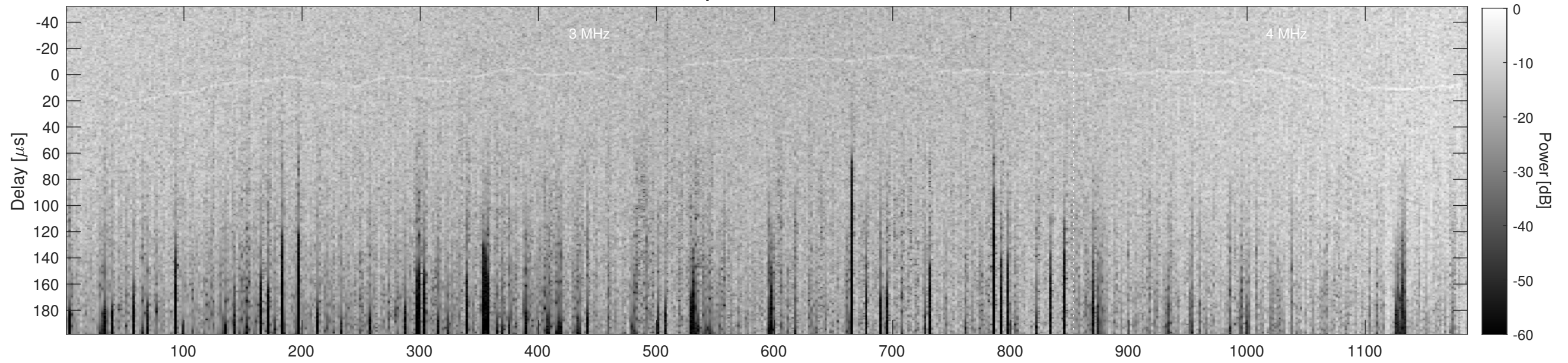
Orbit 10873, Cluttergram
