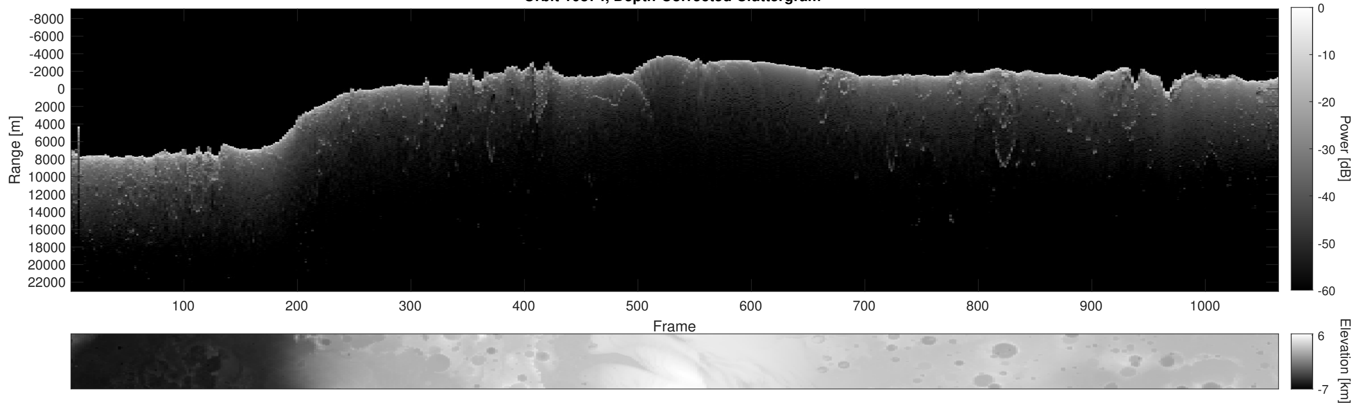
Orbit 10874, Depth-Corrected Cluttergram
