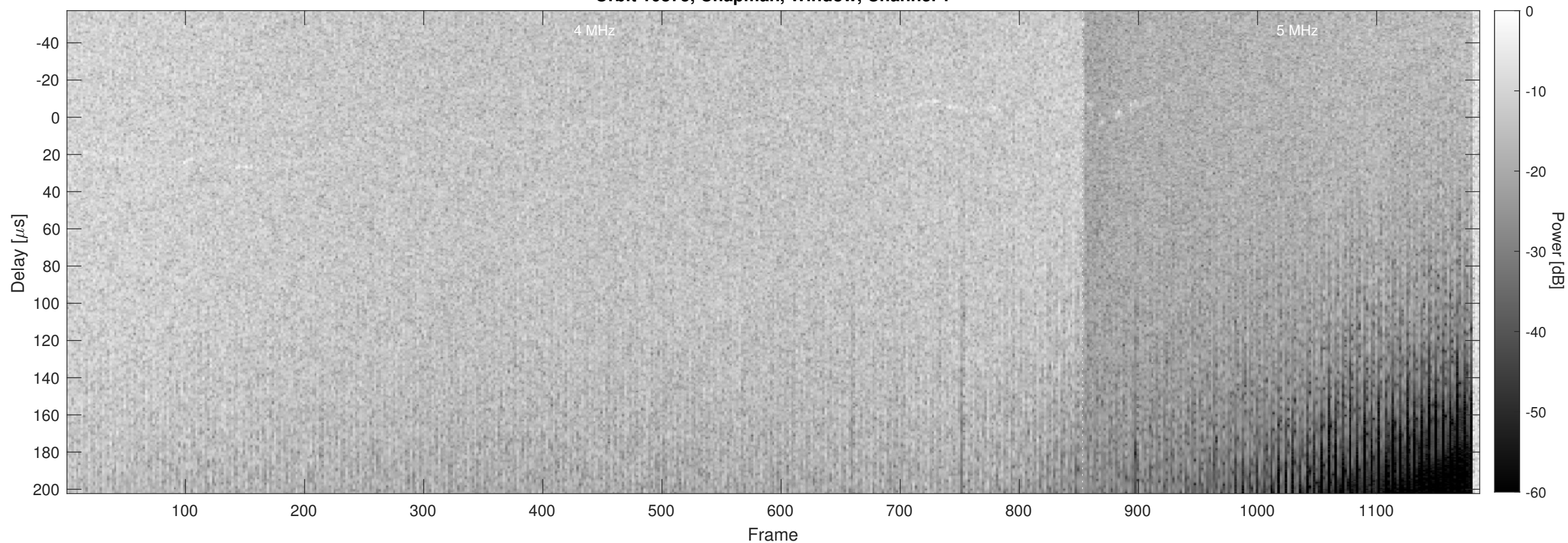
Orbit 10875, Chapman, Window, Channel 2
