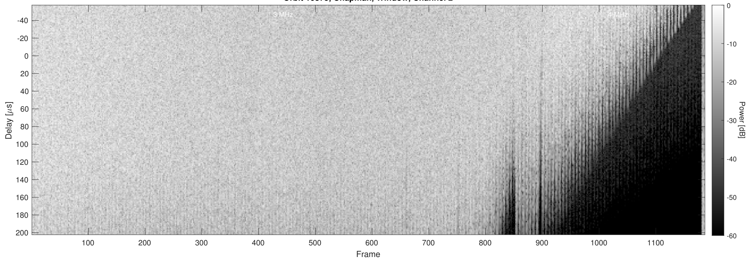
Orbit 10875, Chapman, Window, Channel 2
