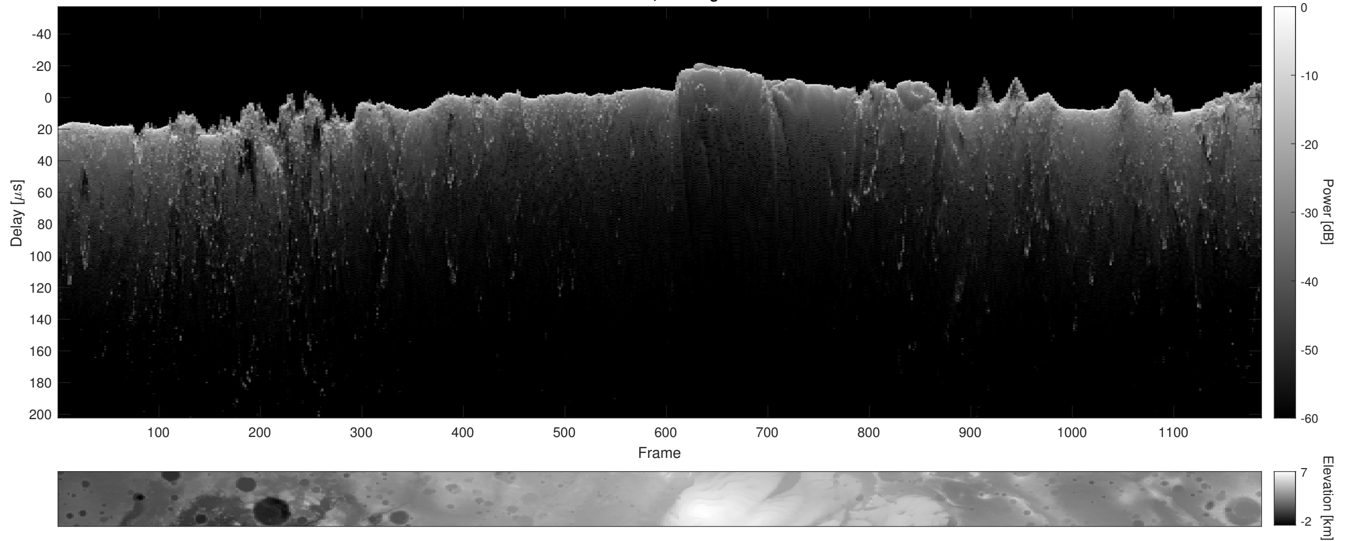
Orbit 10875, Cluttergram
