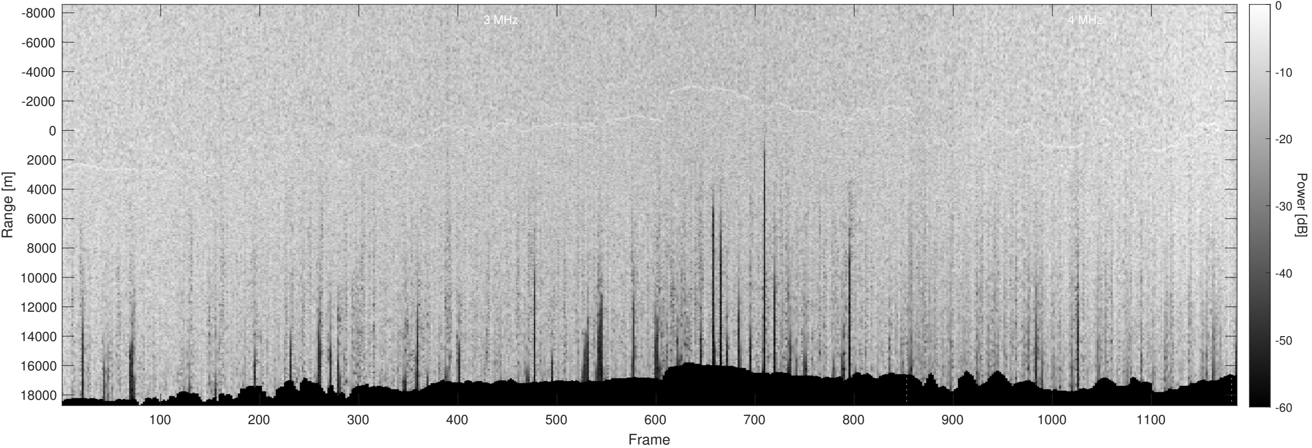
Orbit 10875, Optimized, No Window, Depth-Corrected, Channel 2
