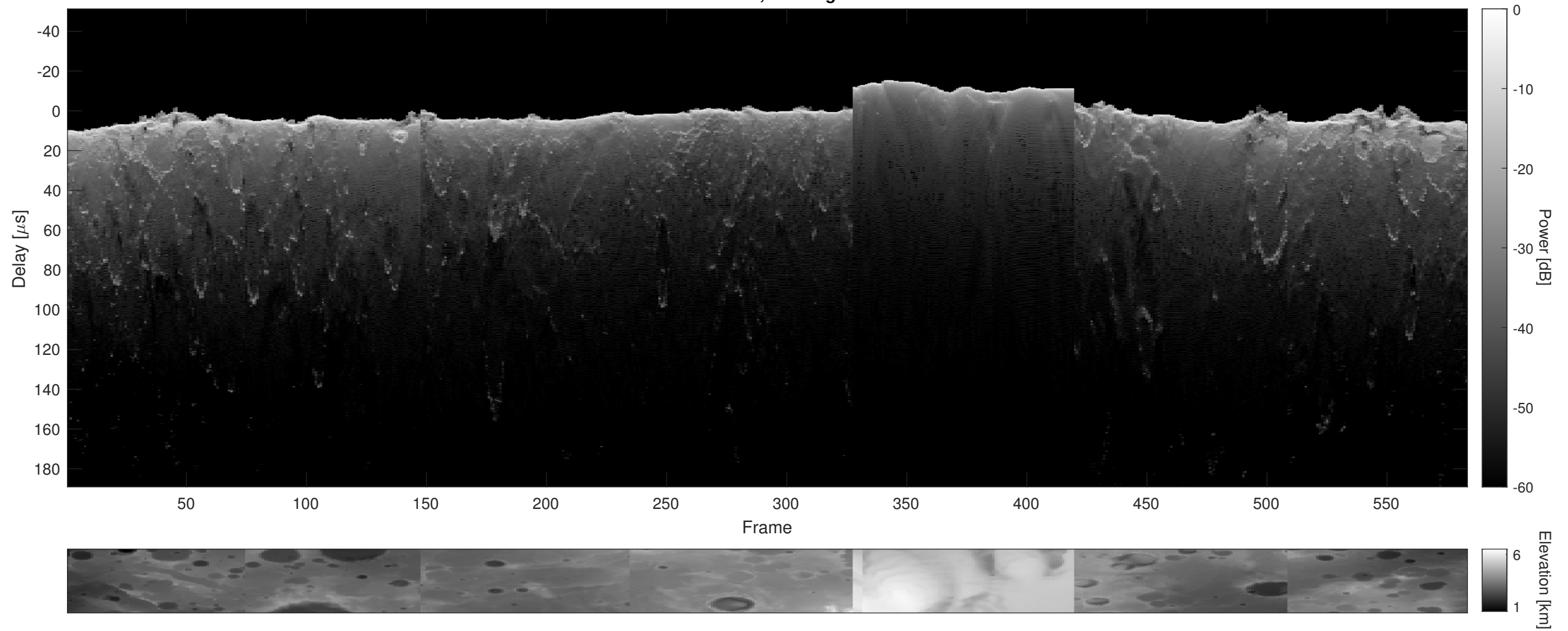
Orbit 10878, Cluttergram
