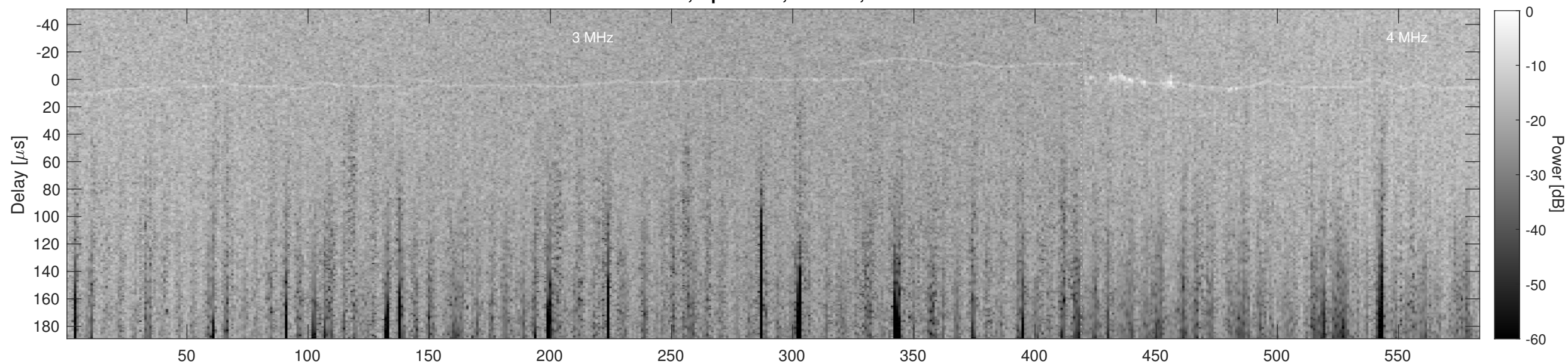
Orbit 10878, Cluttergram
