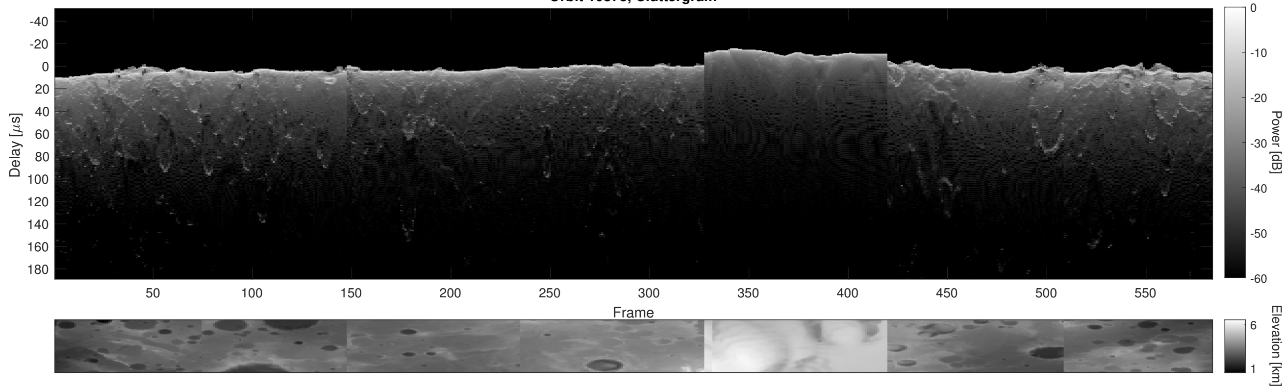
Orbit 10878, Cluttergram
