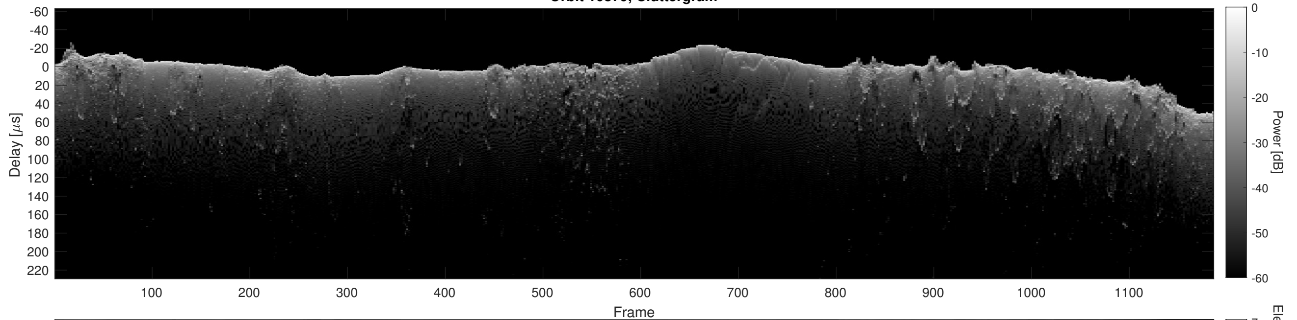
Orbit 10879, Cluttergram
