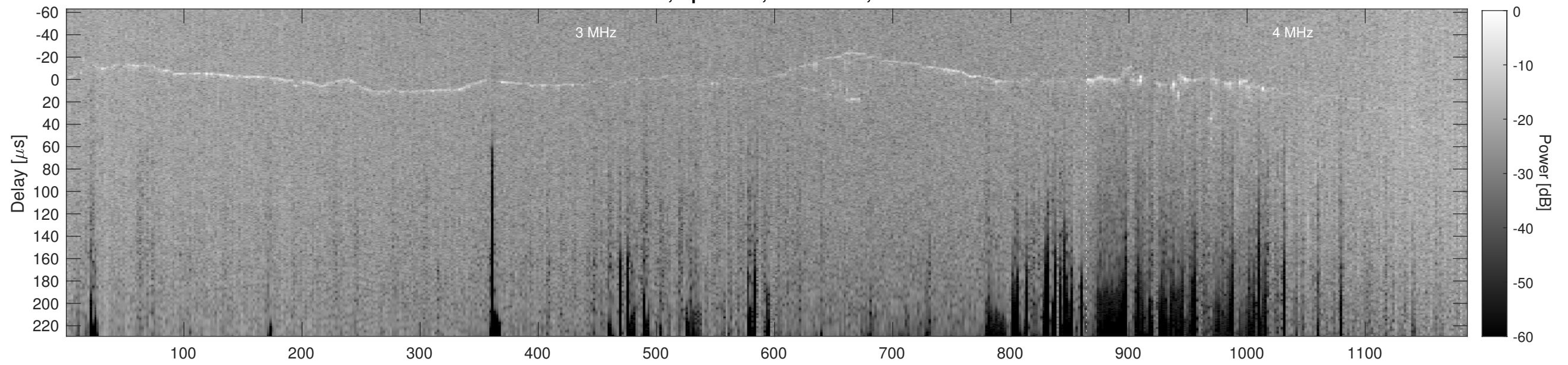
Orbit 10879, Cluttergram
