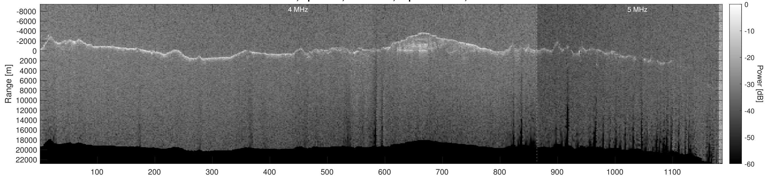
Orbit 10879, Optimized, No Window, Depth-Corrected, Channel 2
