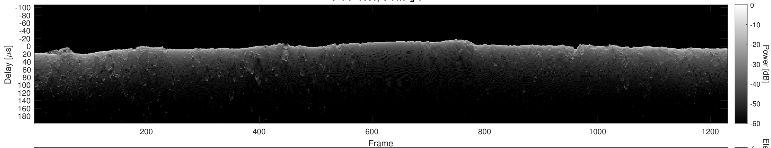
Orbit 10880, Cluttergram
