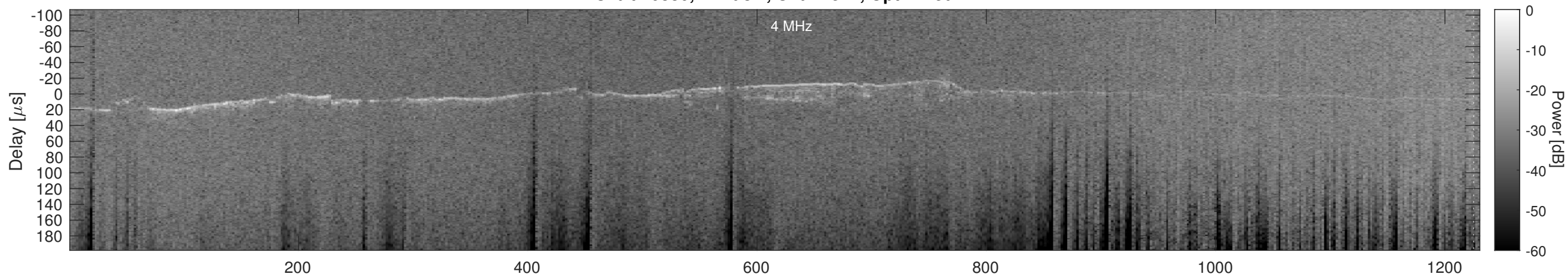
Orbit 10880, Cluttergram
