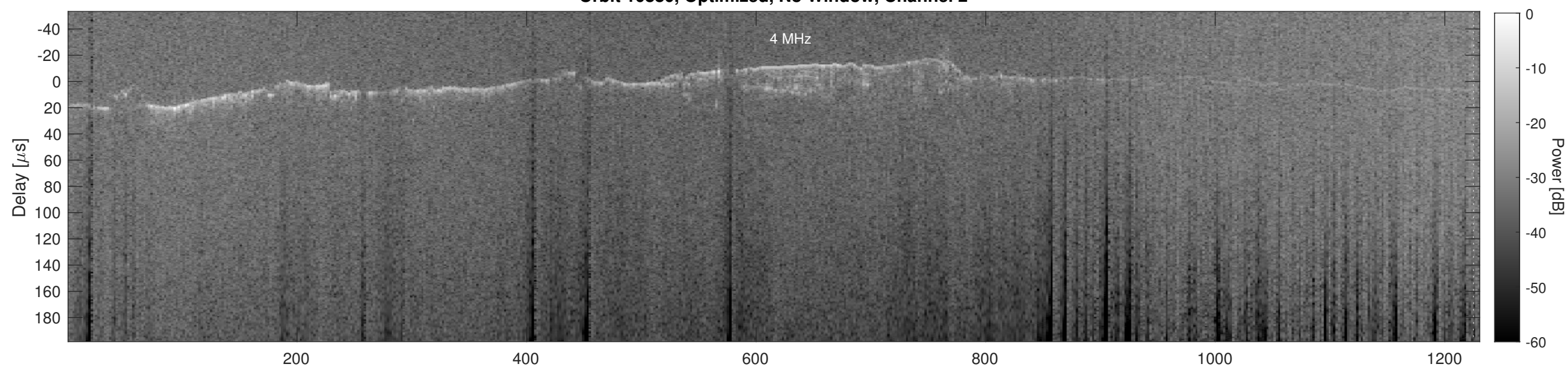
Orbit 10880, Cluttergram
