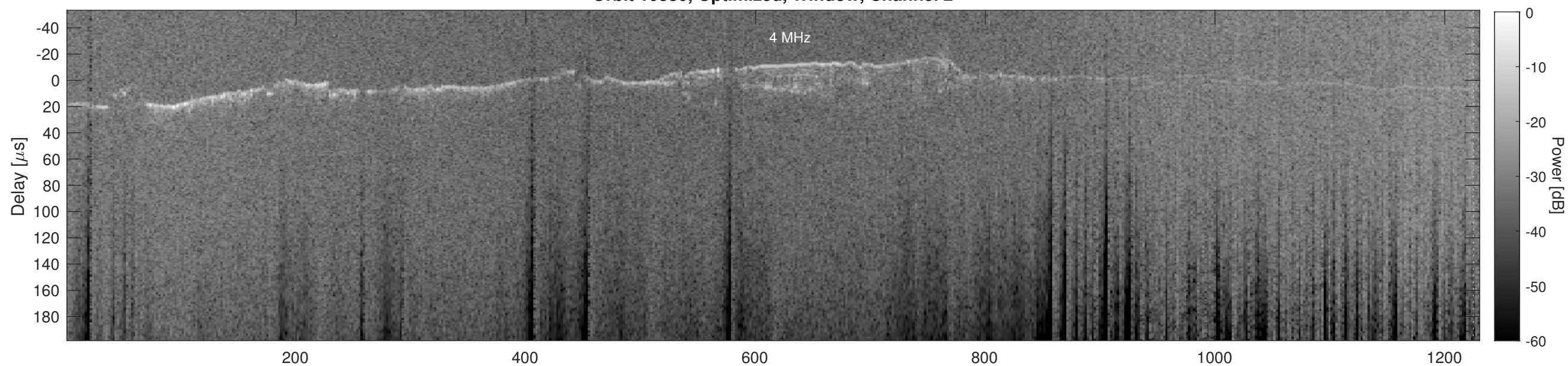
Orbit 10880, Cluttergram
