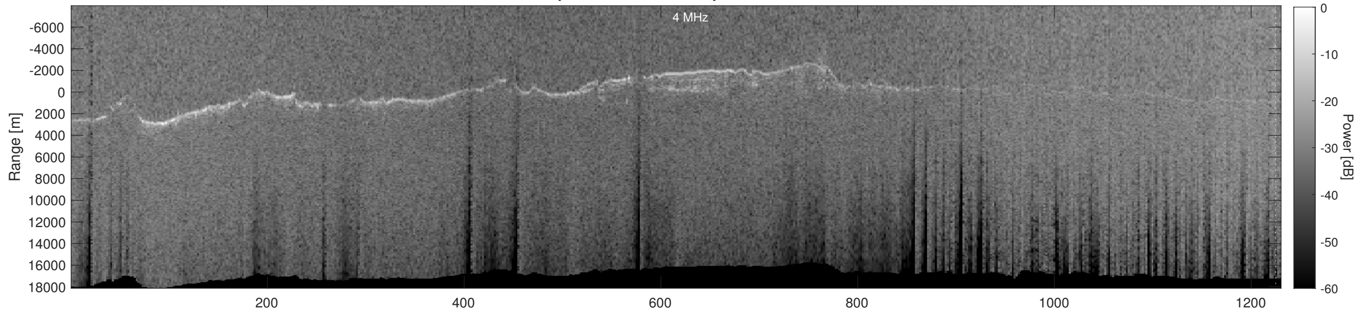
Orbit 10880, Depth-Corrected Cluttergram
