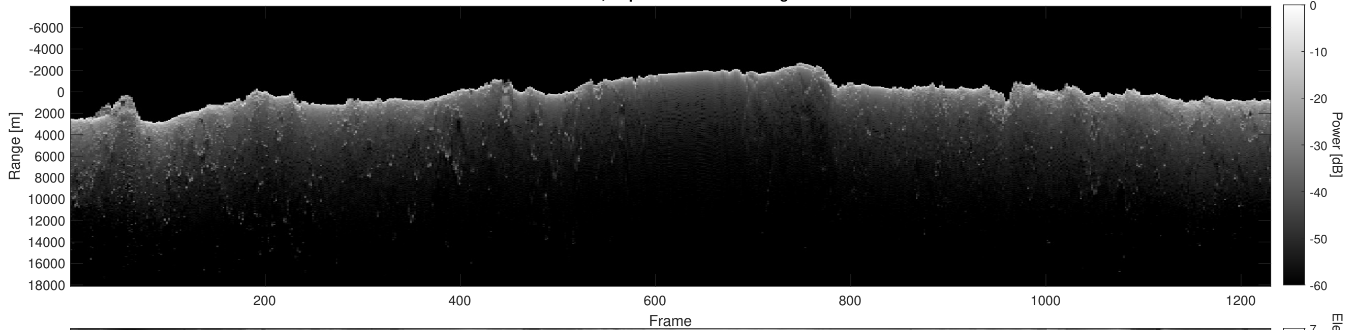
Orbit 10880, Depth-Corrected Cluttergram
