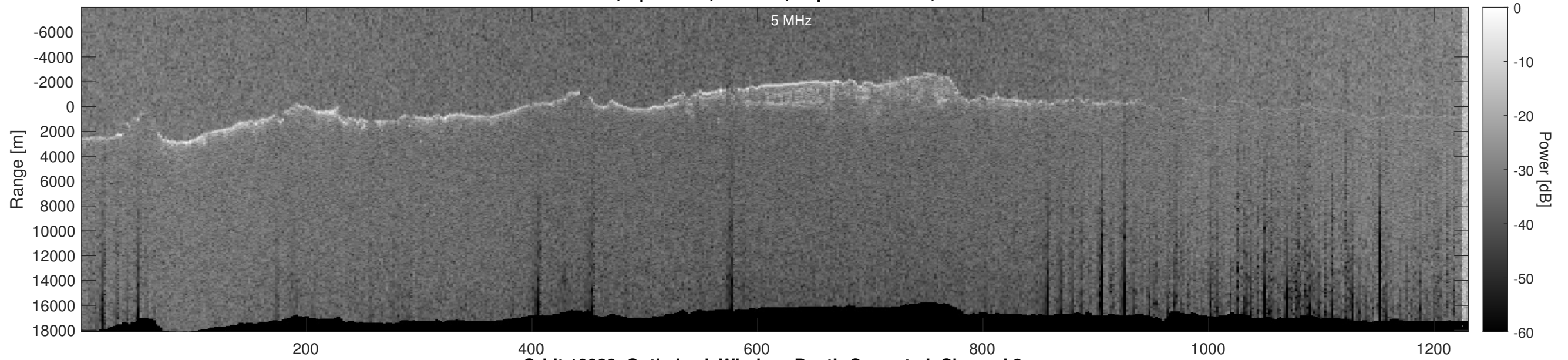
Orbit 10880, Optimized, Window, Depth-Corrected, Channel 2
