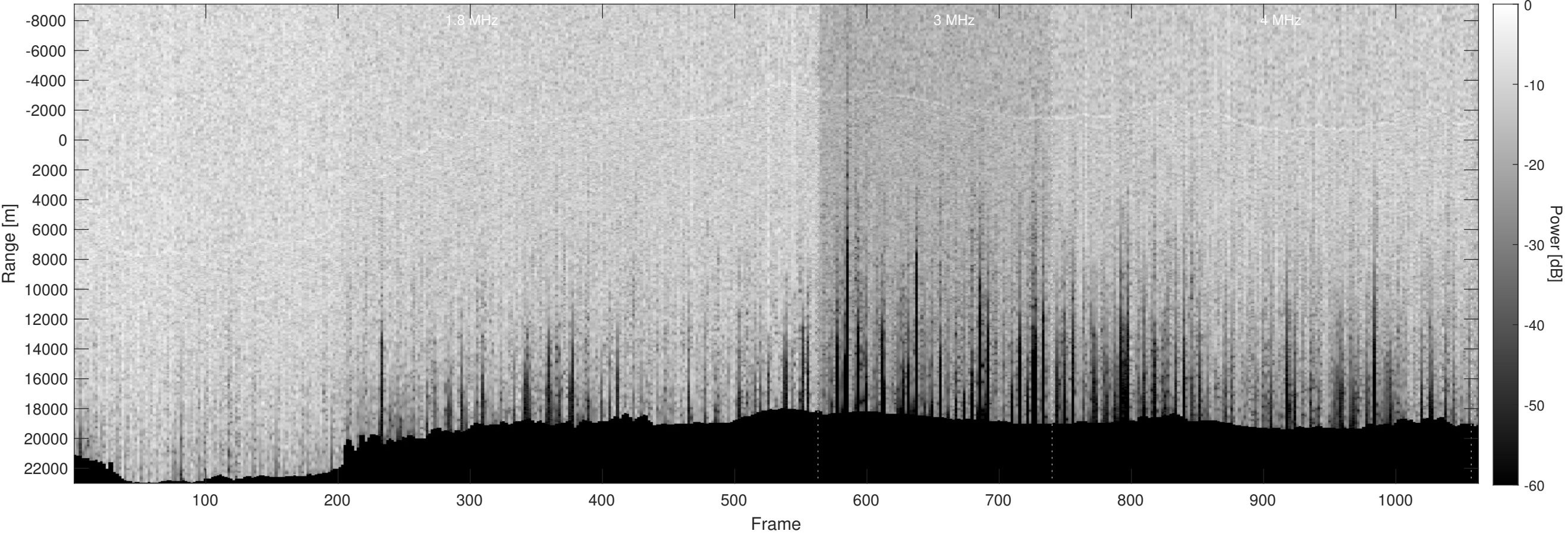
Orbit 10881, Optimized, Window, Depth-Corrected, Channel 2
