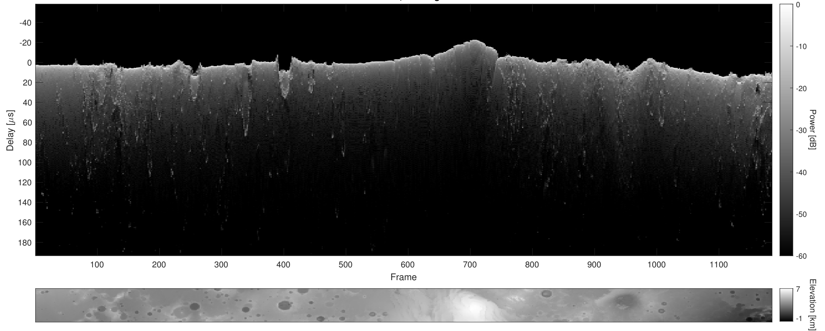
Orbit 10883, Cluttergram
