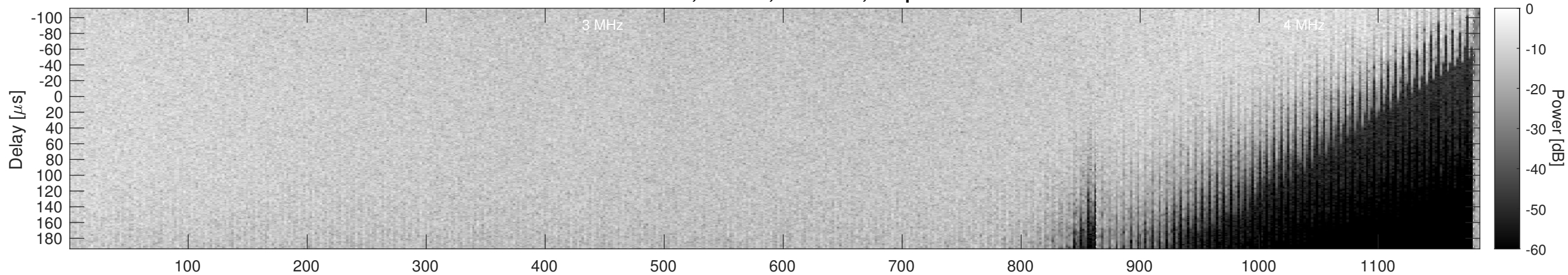
Orbit 10883, Window, Channel 2, Optimized
