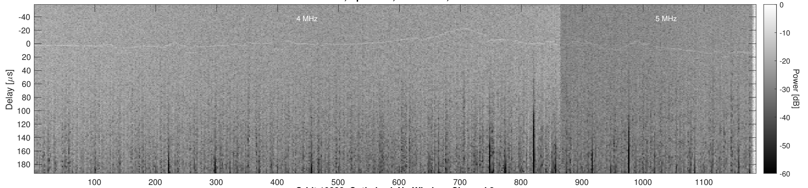
Orbit 10883, Optimized, No Window, Channel 2
