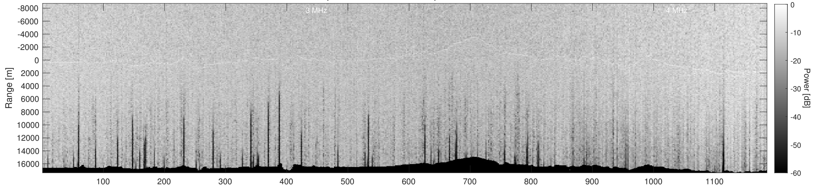
Orbit 10883, Depth-Corrected Cluttergram
