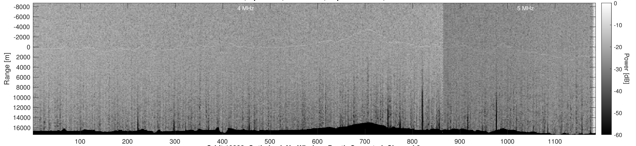
Orbit 10883, Optimized, No Window, Depth-Corrected, Channel 2
