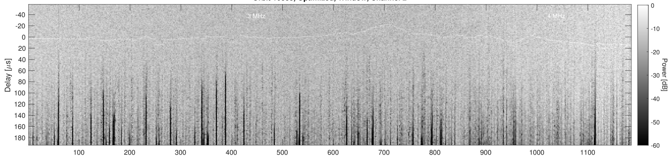
Orbit 10883, Cluttergram
