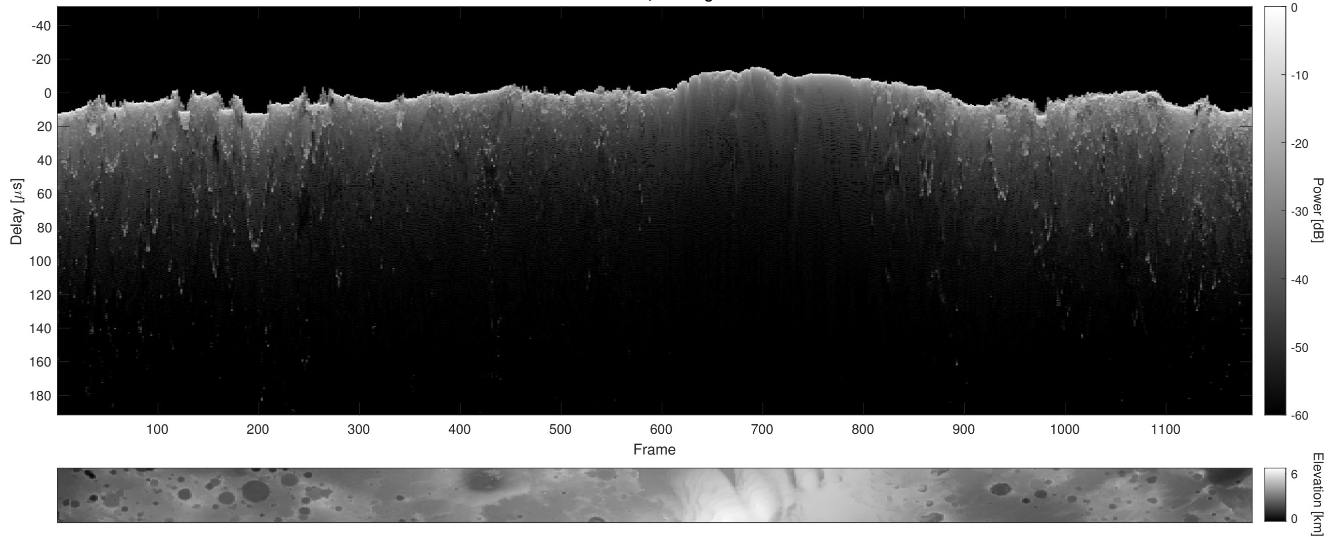
Orbit 10885, Cluttergram
