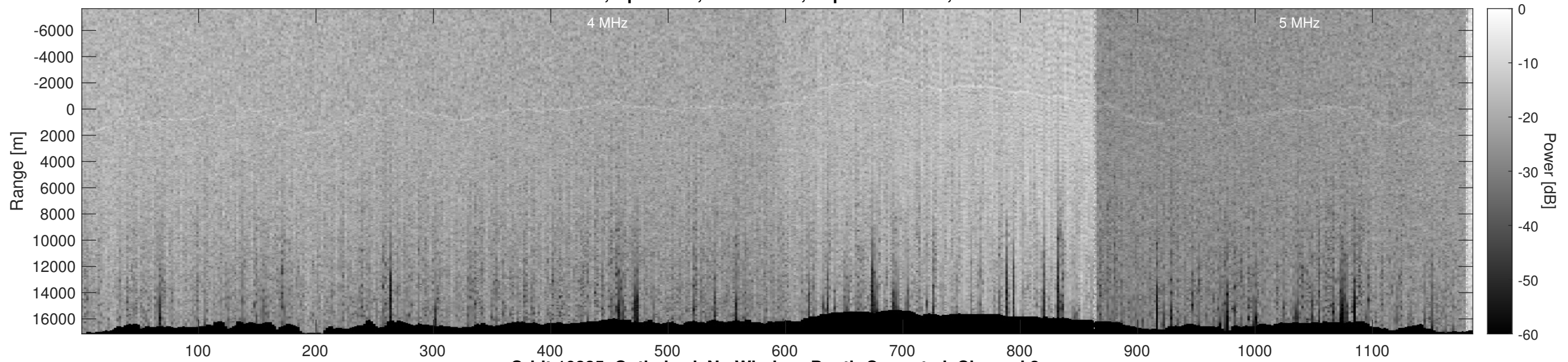
Orbit 10885, Optimized, No Window, Depth-Corrected, Channel 2
