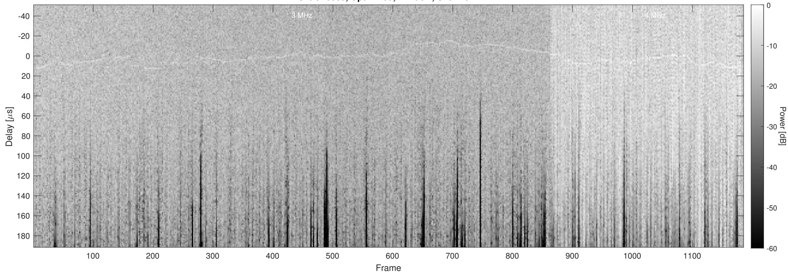
Orbit 10885, Optimized, Window, Channel 2
