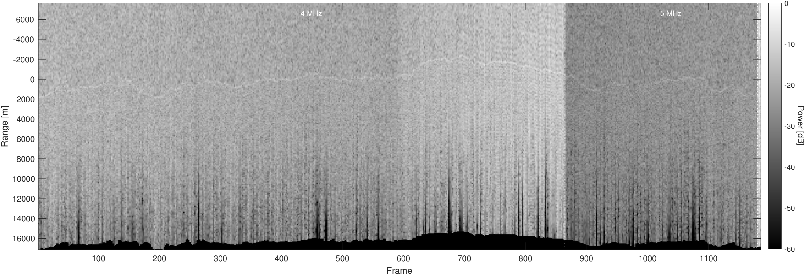
Orbit 10885, Optimized, Window, Depth-Corrected, Channel 2
