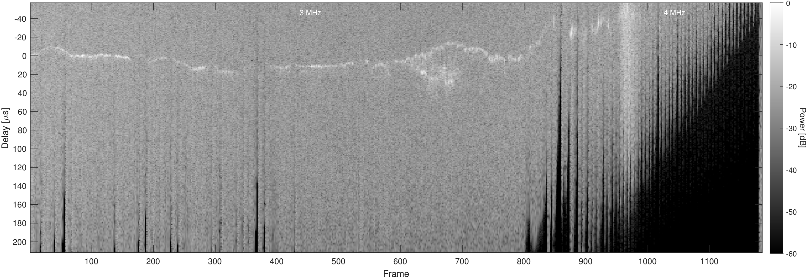
Orbit 10886, Chapman, No Window, Channel 2
