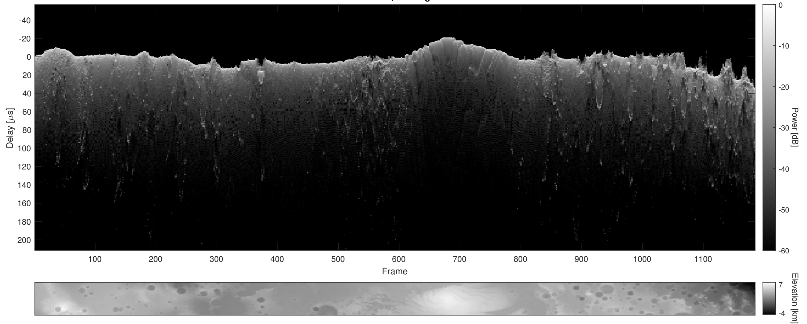
Orbit 10886, Cluttergram
