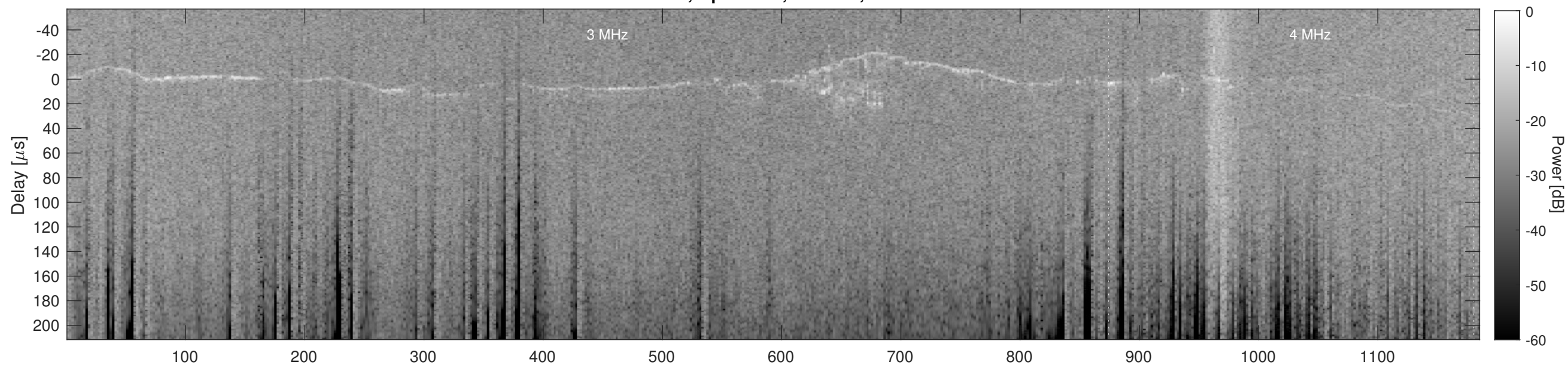
Orbit 10886, Cluttergram
