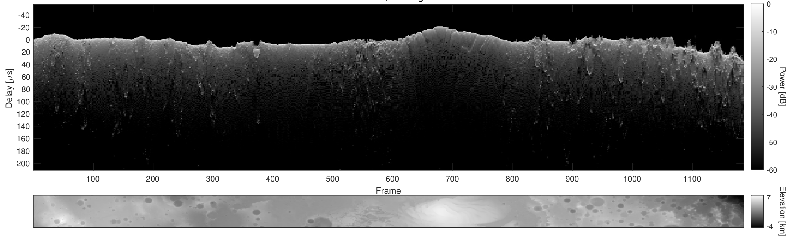
Orbit 10886, Cluttergram
