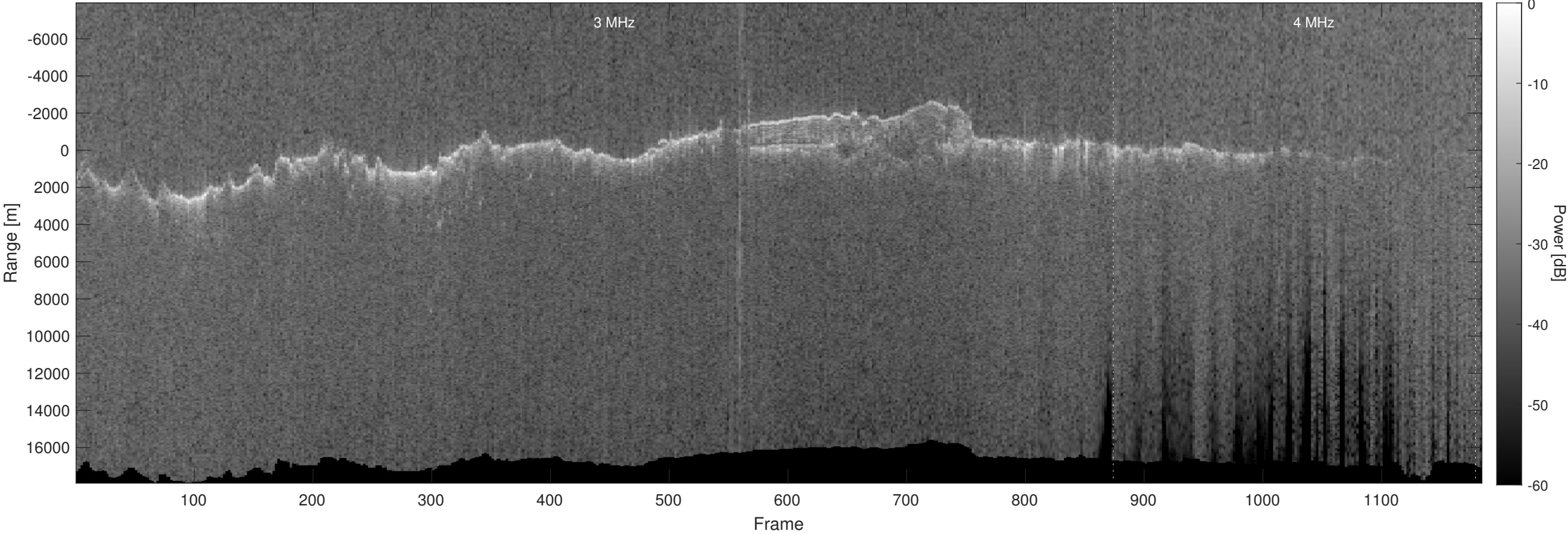
Orbit 10887, Optimized, No Window, Depth-Corrected, Channel 2
