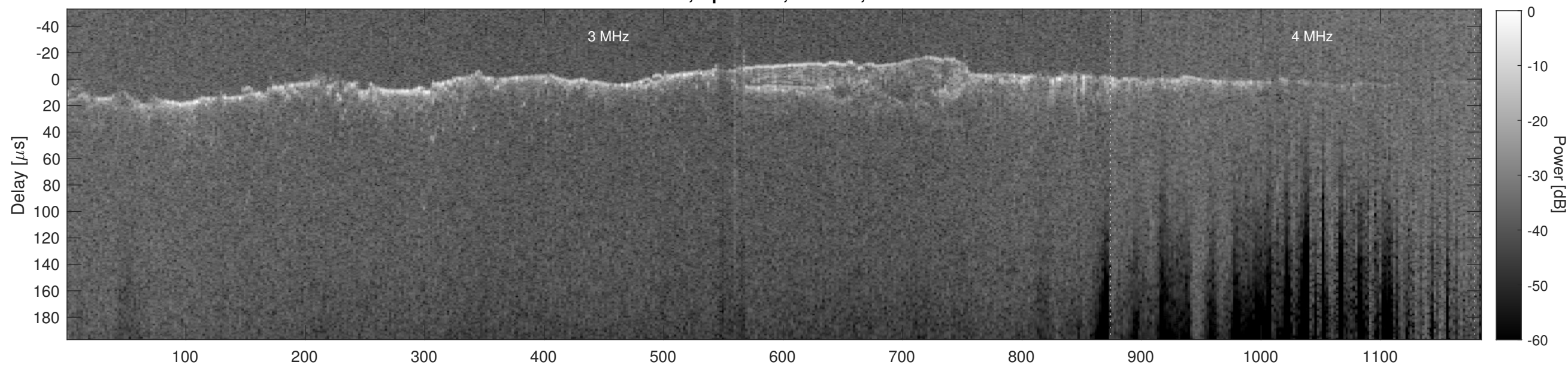
Orbit 10887, Cluttergram
