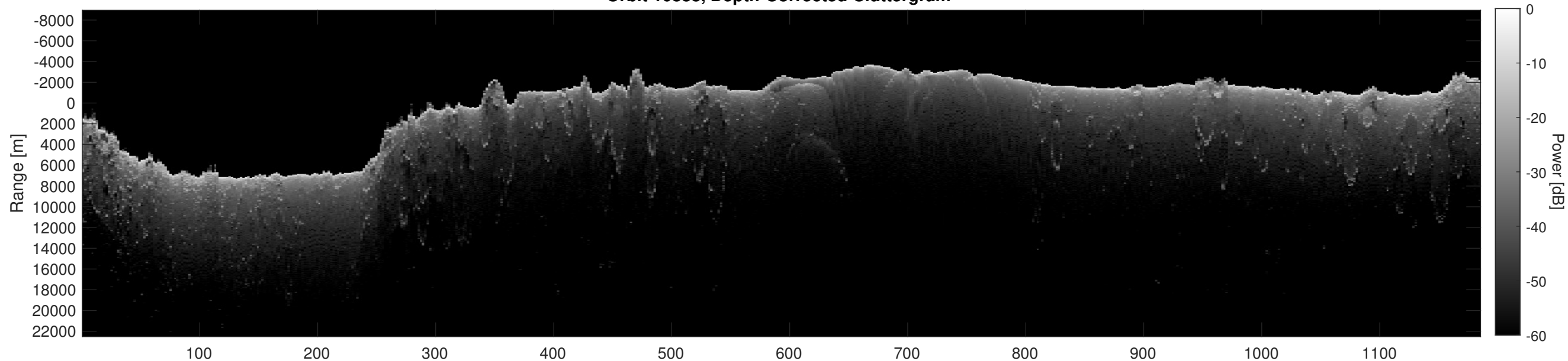
Orbit 10888, Depth-Corrected Cluttergram
