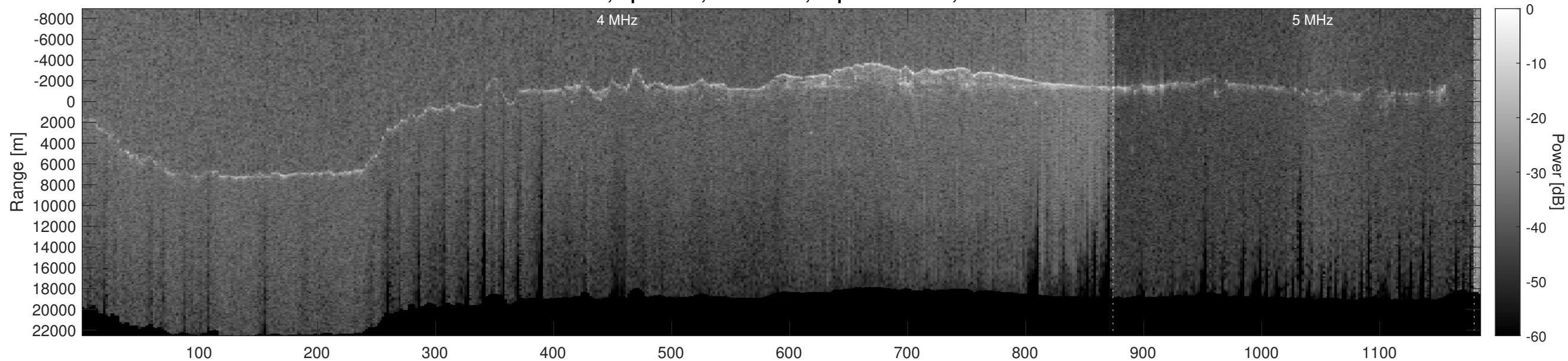
Orbit 10888, Optimized, No Window, Depth-Corrected, Channel 2
