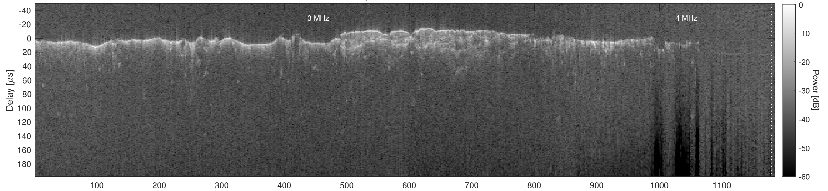
Orbit 10891, Cluttergram
