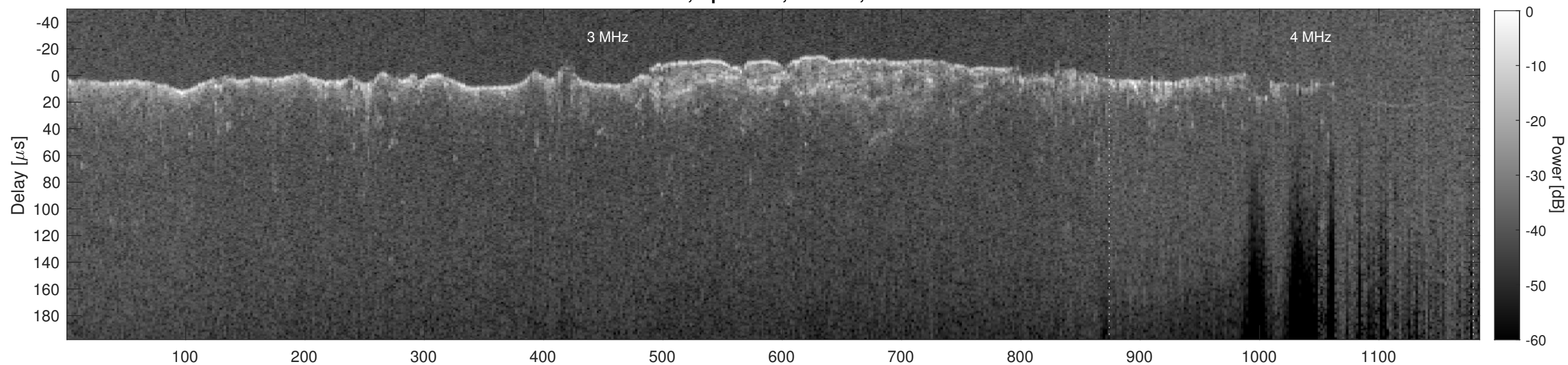
Orbit 10891, Cluttergram
