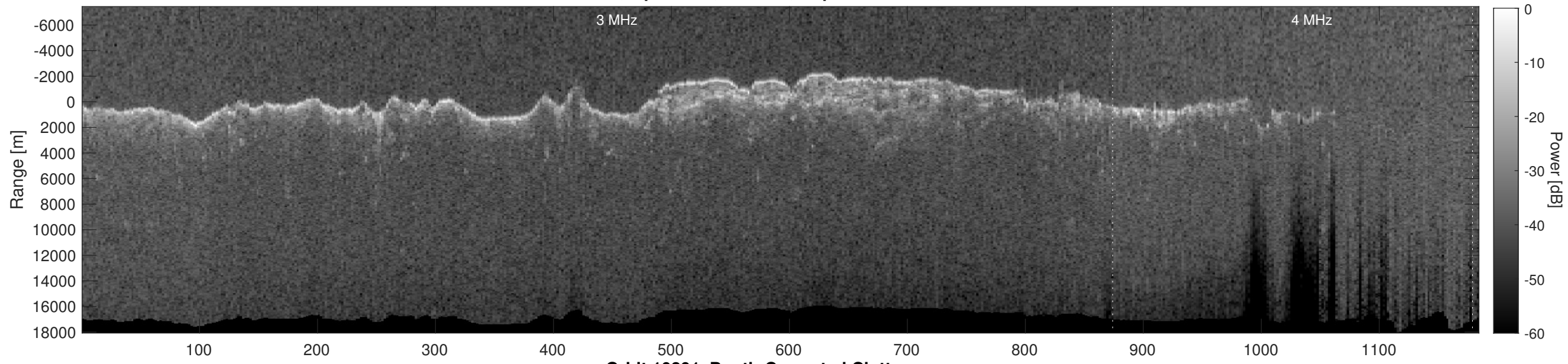
Orbit 10891, Depth-Corrected Cluttergram
