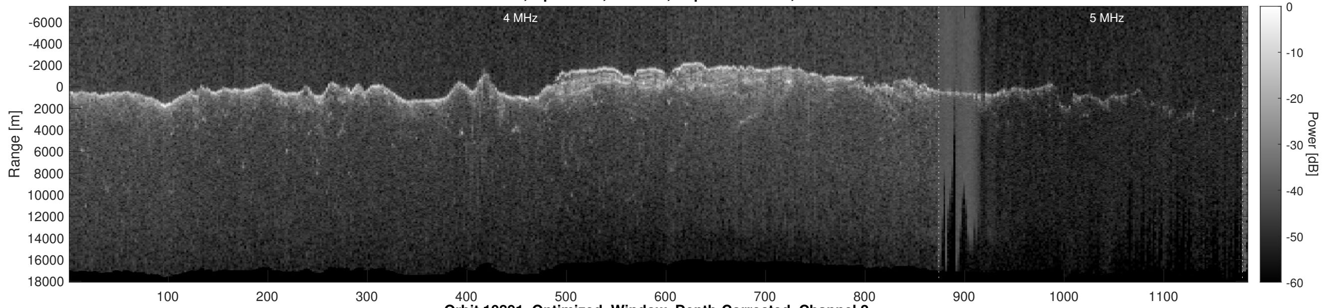
Orbit 10891, Optimized, Window, Depth-Corrected, Channel 2
